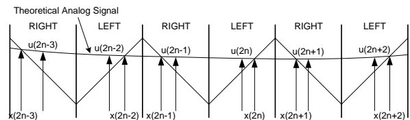
Figure 3 Signal diagram for two-sided PWM
